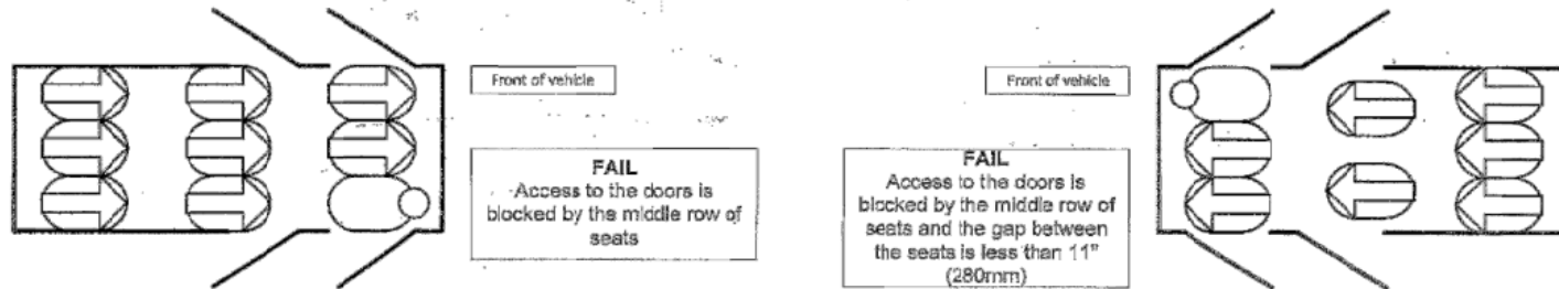
Examples of seating arrangements viewed from above the vehicle
